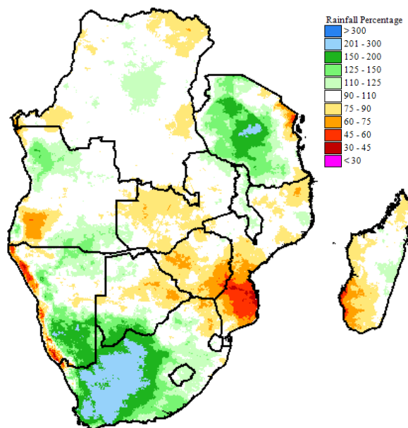
Figure 2. Rainfall for October 2021 to March 2022 as percent of average. Source: CHIRPS, CHIRPS-Prelim
