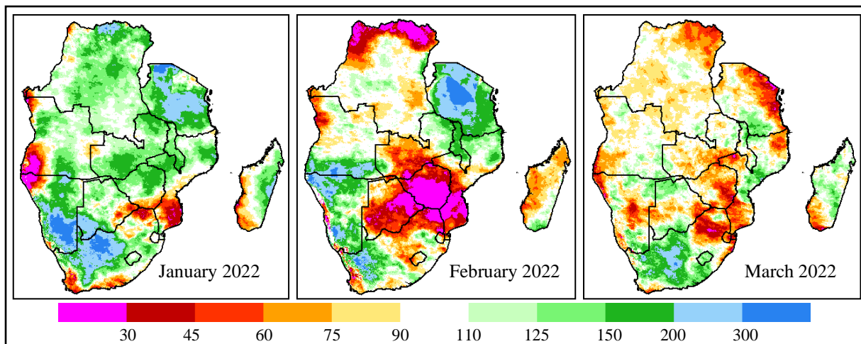
Figure 1. Rainfall for January to March 2022 as percent of average. Source: CHIRPS, CHIRPS-Prelim
