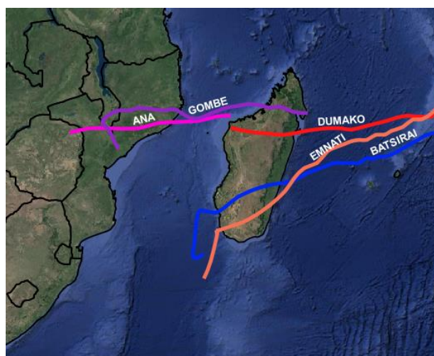
Figure 6. Tropical storms and Tropical Cyclones that have affected southern Africa in the 2021/2022 season. Data Source: IBTRACs, Google Satellite Imagery
