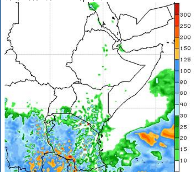
Figure 3. 2 nd Week GFS-Rainfall forecast (mm), valid December 12 - 18, 2017
